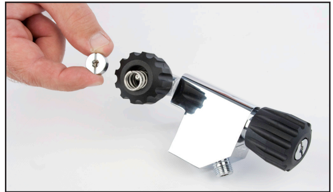
Remove the lock nut, spring and knob.
