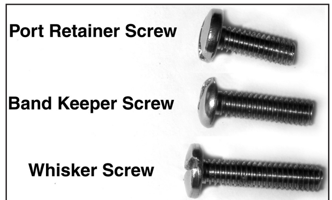
Note that the screws used for the port retainer, band keeper and whisker have a similar appearance, but that all are different lengths. They are not interchangeable.
